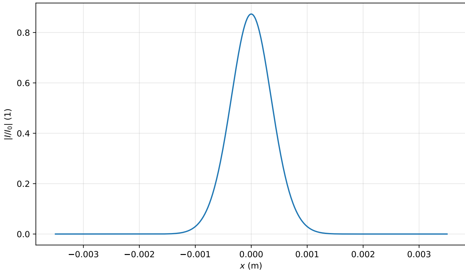
Intensity profile I(x, y = 0, z = 1.035m)/I_0 , P_{in}=0.2P_{cr} , artificial time
